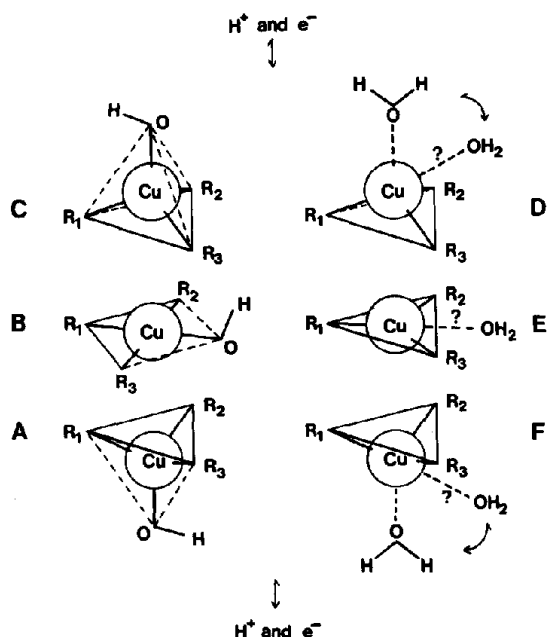
Fig.3. Suggested type of mechanism for coupling electron transfer to hydroxide translocation at the \text{Cu}_A or \text{Cu}_B centre of cytochrome oxidase. R_1 , R_2 and R_3 represent amino acid ligands in the osmotic barrier domain of the oxidase, the i site being above the plane of these ligands, and the o site being below it. Diagrams A–F represent the sequence of states in the working configurational cycle. In passing back from the i to the o site at the Cu centre, the \text{H}_2\text{O} may or may not travel in close proximity to the copper atom, as indicated by the question marks in diagrams D, E and F. The circle round Cu does not represent the size of the Cu atom.
